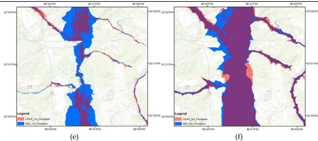
Figure 5. NED-HAND & LiDAR-HAND Inundation Extent Comparison
